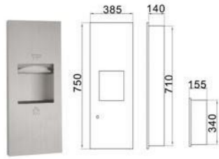
Model : YS-5856 Paper holder with rubbish box 手紙箱連垃圾箱 Size: 385x750x140mm
