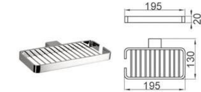
Model: BG-7802B2 Soap basket 肥皂網
