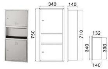
Model : YS-5831 Paper holder with rubbish box 手紙箱連垃圾箱 Size: 340x750x140mm
