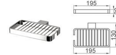
Model: BG-7802B1 Soap basket 肥皂網
