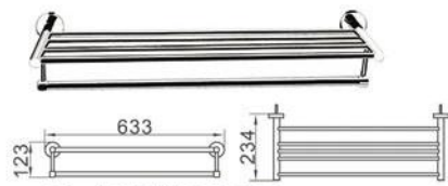
Model: BW-68880B Bath towel rack 浴巾架
