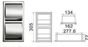
Model : YS-5802 Name: Recessed double paper holder Main Material: 304 stainless steel Color: polish finished satin finished 入牆雙廁紙架
