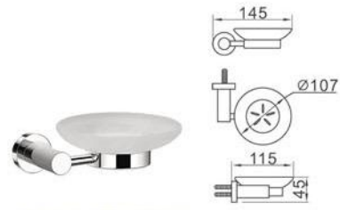
Model: BW-68590 Soap dispenser 肥皂架
