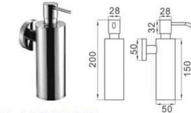
Model: BW-68518 Wall mounted soap dispenser 皂液器
