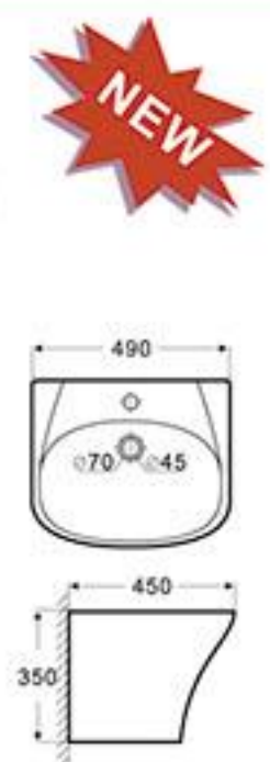
JH-5600C 半柱盆 尺寸: 490x450x350 毫米 Half Pedestal Basin Size: 490x450x350mm
