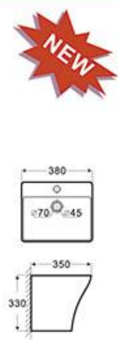
JH-5400C 半柱盆 尺寸: 380x350x330 毫米 Half Pedestal Basin Size: 380x350x330mm
